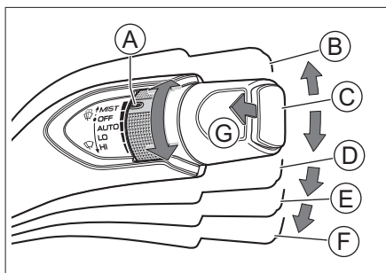
Ⓐ Anillo selector
