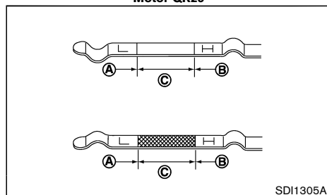
Motor MR20
