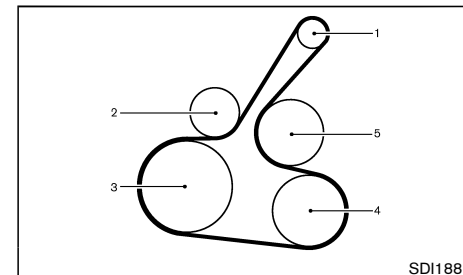
Motor MR20DD
