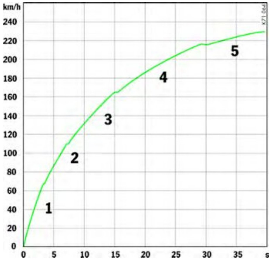
Boxster: Acceleration diagram Manual transmission. Values have been determined at DIN empty weight and with a 50 % load without additional equipment.
